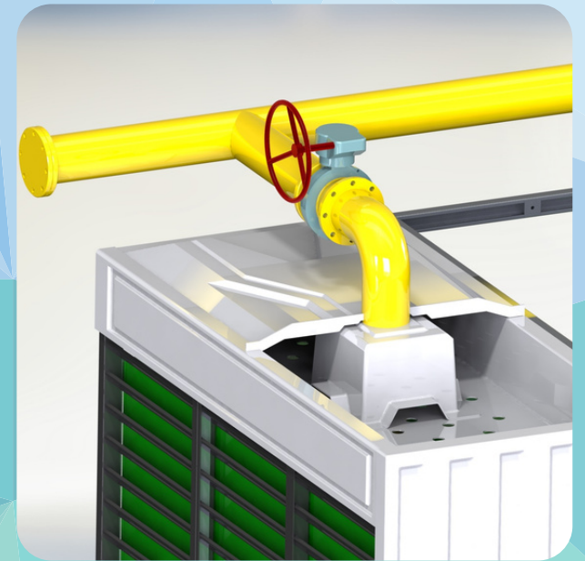
FRP. Distribution basin
